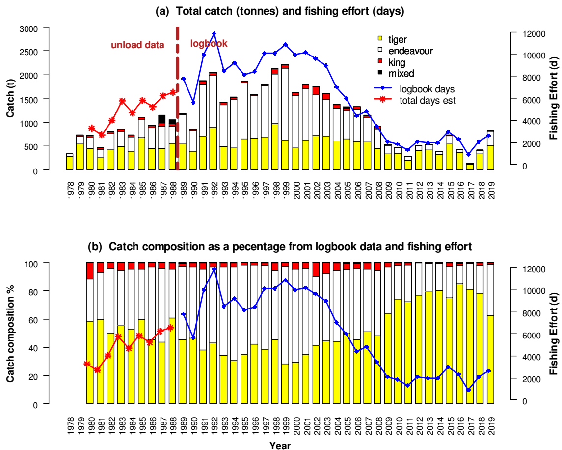
Figure 3 (a) Total catch in tonnes from unload data (1978–1988) and logbook day (1989–2019). Fishing effort (days) is from logbook data (1989–2019) and the “total days estimate” for 1980–88 is from logbook data adjusted by the logbook coverage. (b) Catch composition as a percentage from logbook data. Note that the 1980–1988 logbook data is from a subset of the fleet.
