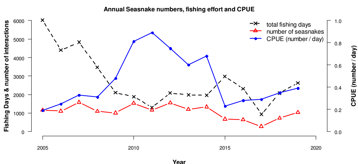
Figure 11. The annual number of interactions (reported in logbooks) with seasnake (red line with triangles) plotted against the number of fishing days (black dotted line with x) and both are scaled to the left y-axis. The solid blue line with circles is the Rate of interactions with seasnake (i.e. CPUE) expressed as number of interactions per fishing day and is scaled to the right y-axis.
