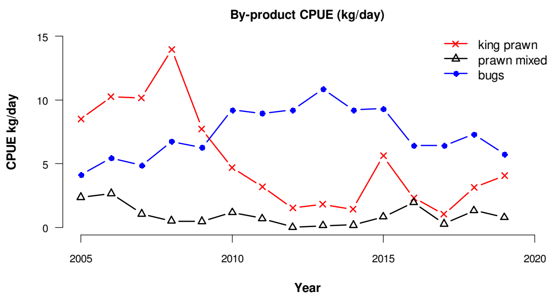
Figure 13 By-product CPUE (kg/d) for king prawn (the combined red spot king prawn + king prawn mixed columns listed in table 3), prawn mixed and bugs for the years 2005 to 2019.
