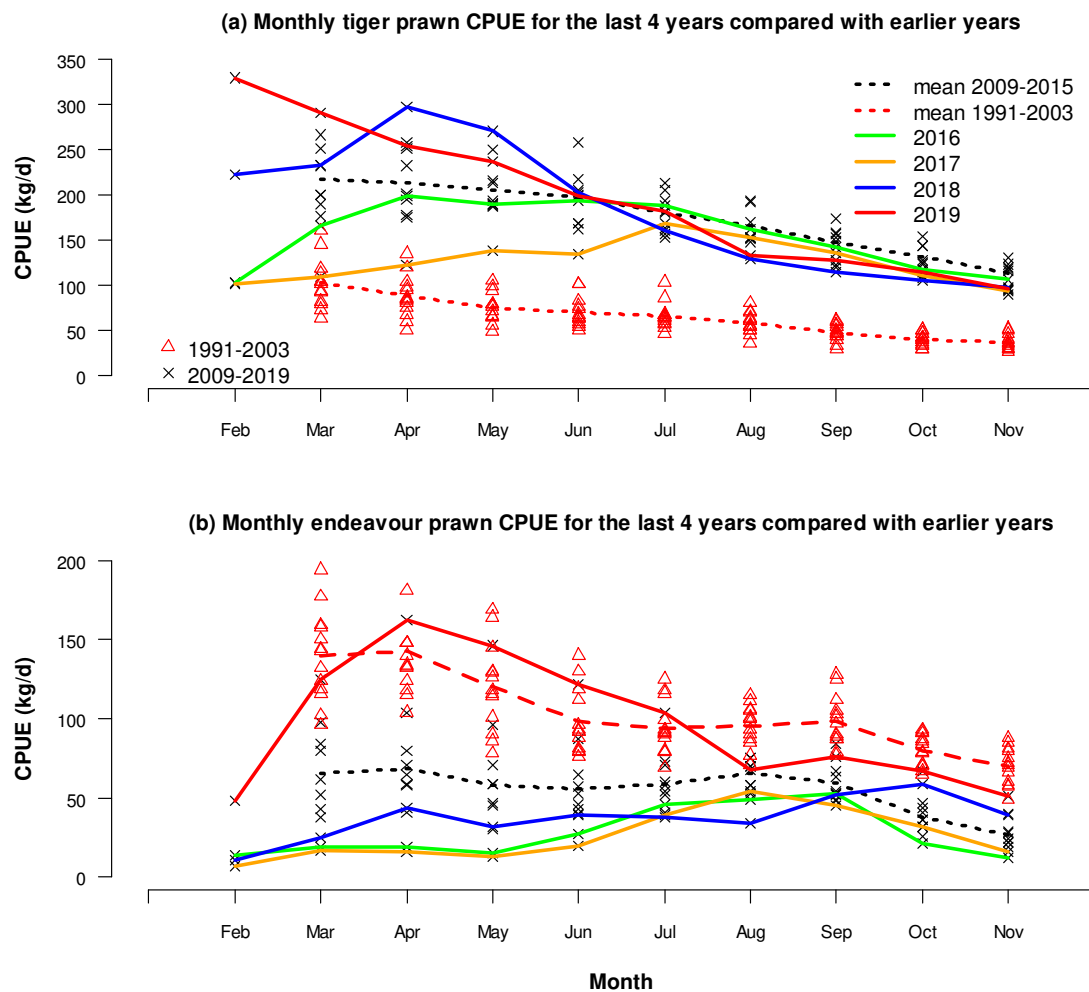
Figure 10 Catch Per Unit of Effort (CPUE) as kilograms per day for (a) tiger prawn and (b) endeavour prawn. The CPUE for each month of the years 2016-2019 is compared with the distribution and mean of the monthly CPUE for 2009-2015 and the years of highest fishing effort (1991-2003). The point symbols ( \times and triangles) show the individual monthly CPUE for the two time periods.
