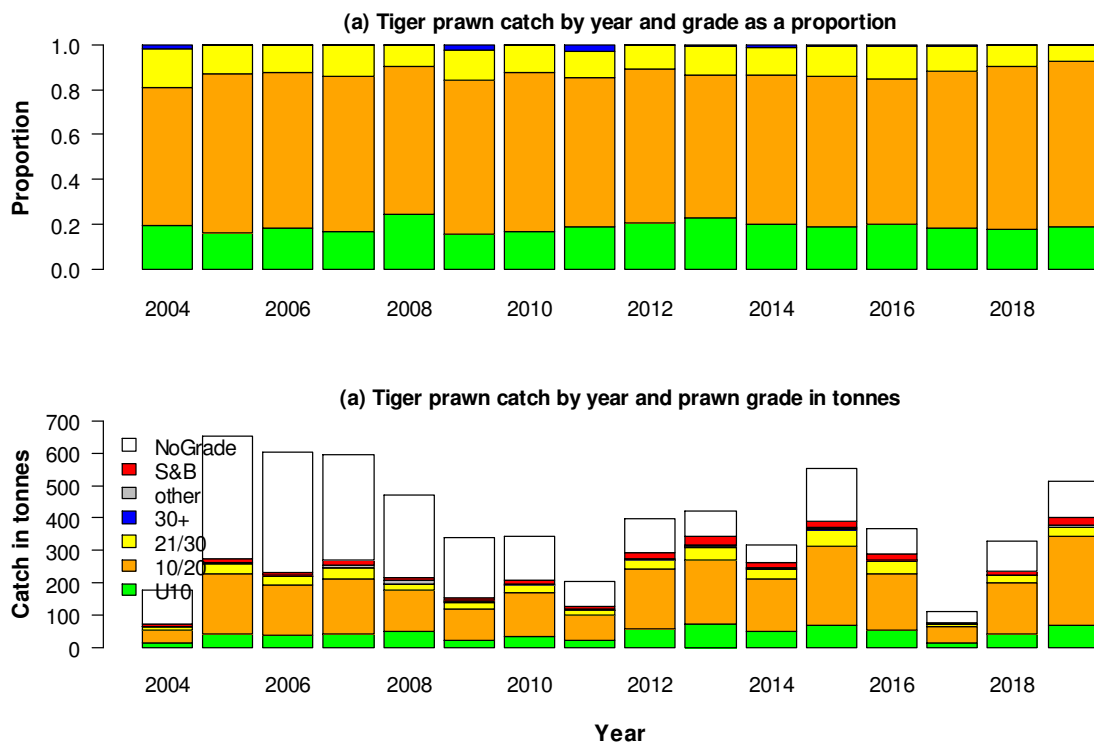
Figure 11 (a) Tiger prawn grades as a proportion for each year. (b) Tiger prawn catch in tonnes by grade. Note: that 2004 is only partial data due the phasing in of the new logbook format that included grade.
