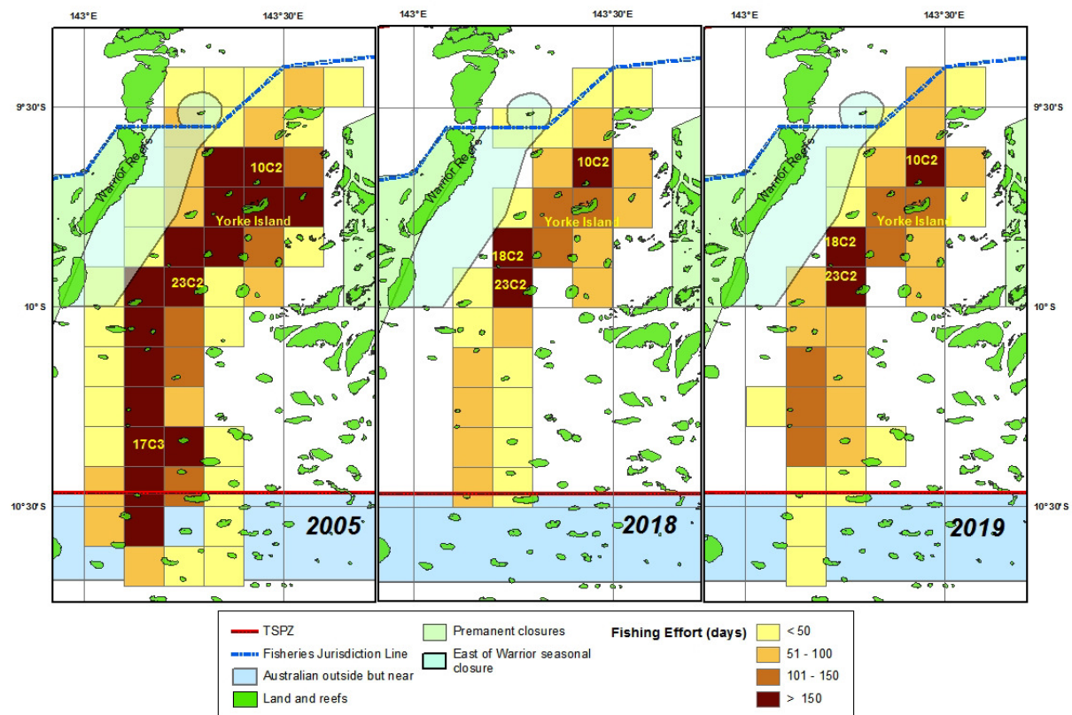
Figure 6 Effort distribution (fishing days across all boats) within the TSPF for the 2005, 2018 and 2019 fishing seasons by 6-minute grid.
