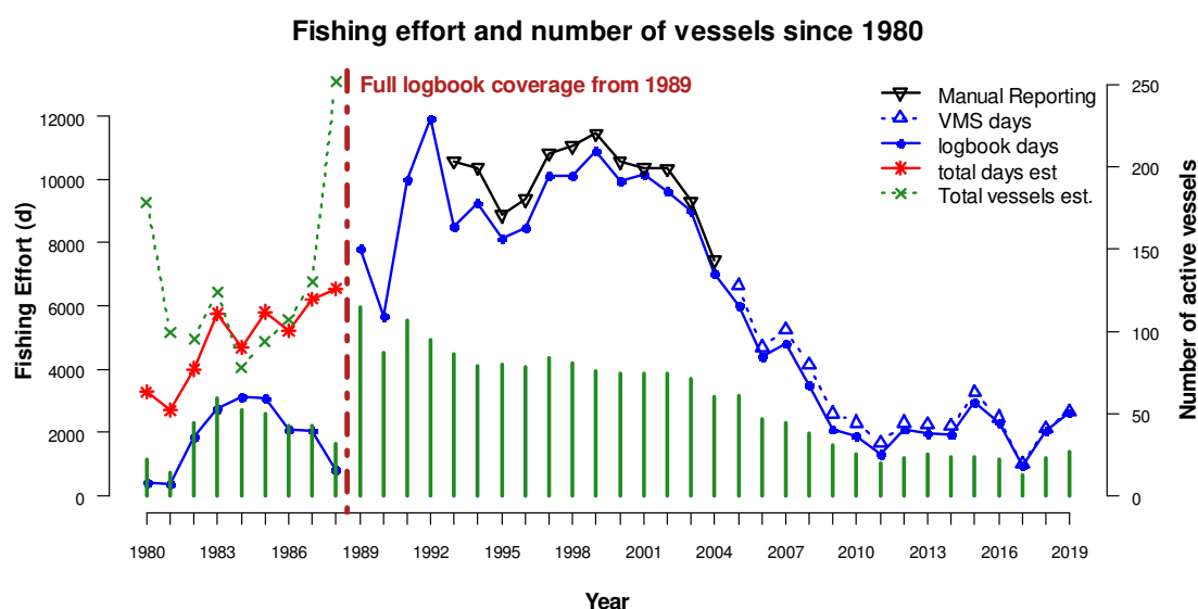
Figure 2 The total days fished in the Torres Strait Prawn Fishery since 1980; displayed as manually reported fishing days (1993-2004), quota usage from the Vessel Monitoring System (2005-2019), logbook days (1980-2019) and “Total Days est.” (1980-1988; from logbook days adjusted by the logbook coverage of the total catch). The green vertical lines show the number of active vessels each year based on the logbook data. The yearly estimates of all active vessels during 1980-88 are plotted as “Vessel Number est”. Note there was only partial coverage of the fishery by logbooks prior to 1989.
