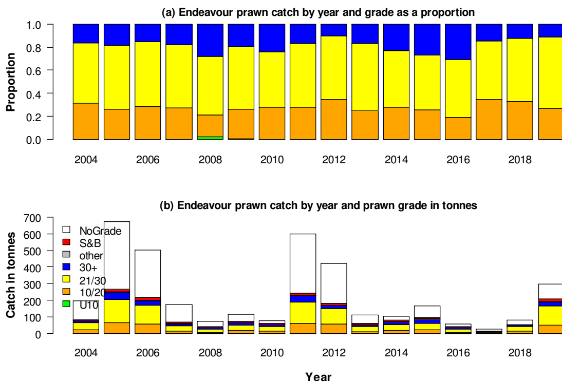
Figure 12 (a) Endeavour prawn grades as a proportion for each year. (b) Endeavour prawn catch in tonnes by grade. Note: that 2004 is only partial data due the phasing in of the new logbook format that included grade.
